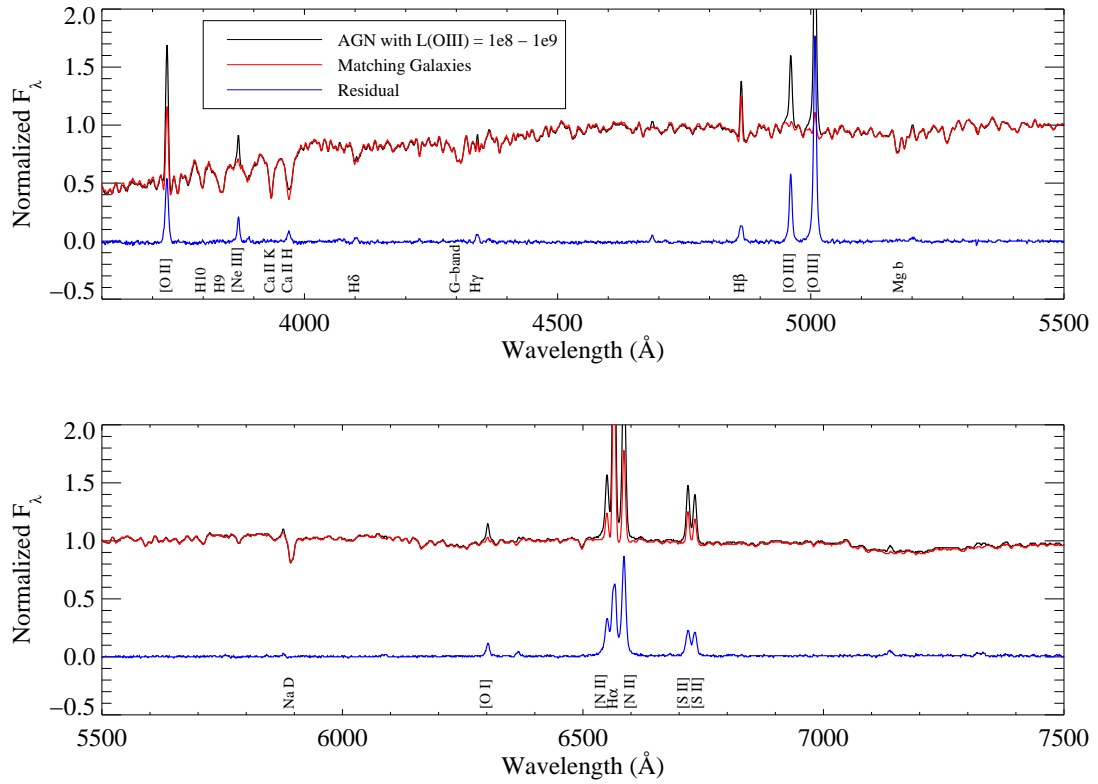
Figure 4: A comparison of the stacked spectra of 500 AGN with [OIII] line luminosities in the range 10^8 - 10^9 solar (black) with the stacked spectra of a set of matching galaxies (red). The blue line shows the residual when the galaxy spectrum is subtracted from the AGN spectrum.
